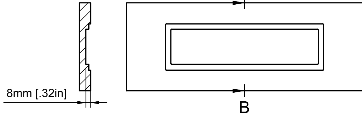
Section B-B (1:4)
